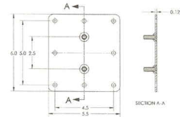
Figure 1 - Roof Mount Base Plate
