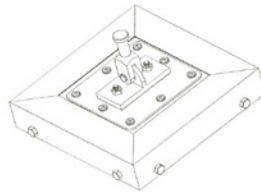
Figure 3 - Pullout Test Fixture
