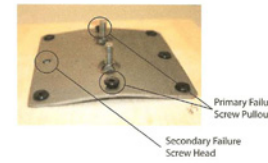
Figure 5 - Typical Pullout Test Result
