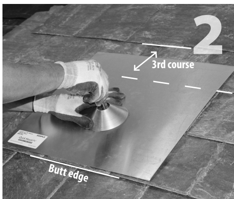
To mark the location of the QB-1, position the bottom edge of the flashing flush with or just above the butt edge (drip) of the slate, the top edge extended up under the 3rd course, and the cone centered over your rafter centerline.
