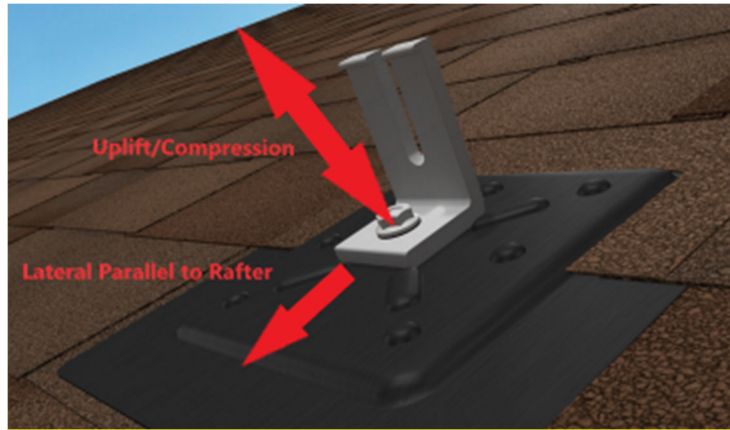
Figure 1: EcoFasten 44-R and Applied Loading Directions
